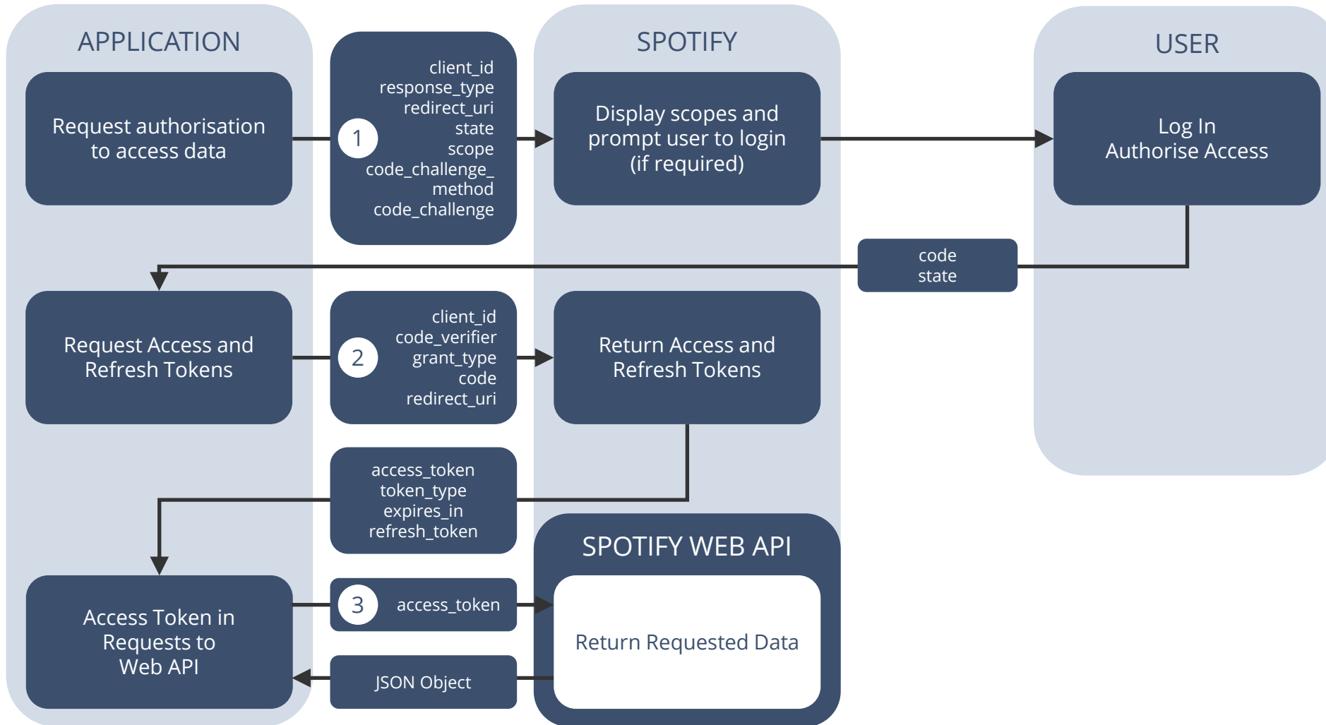
Authorisation Code with Proof Key for Code Exchange Flow
